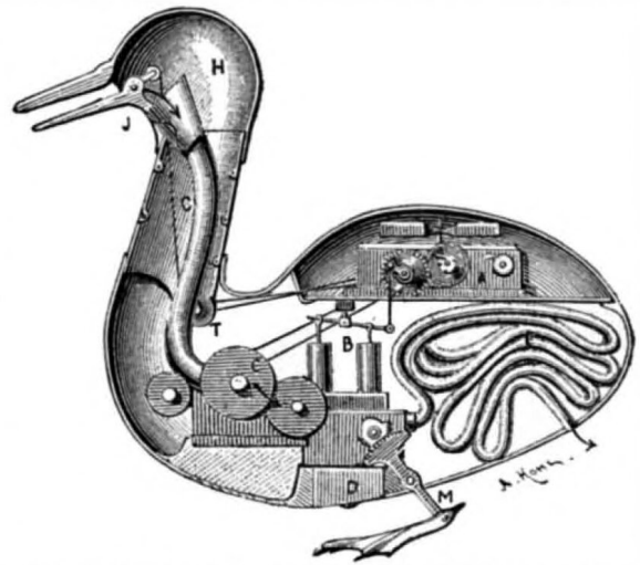
INTERIOR OF VAUCANSON'S AUTOMATIC DUCK.
